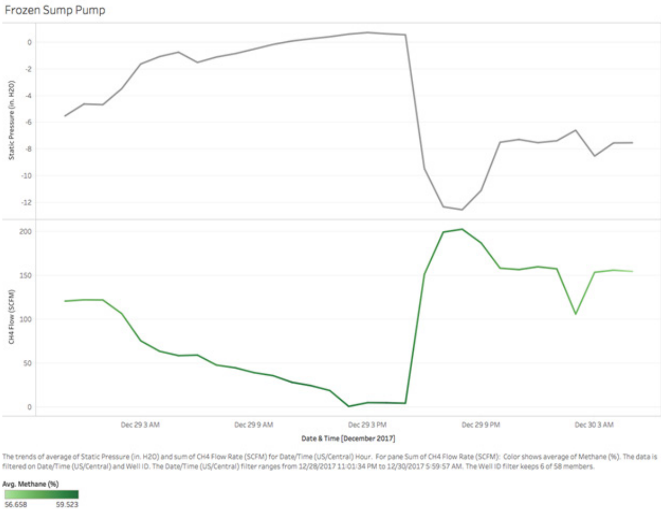
Figure 4: Loss of static pressure due to a frozen sump pump and resulting loss of flow. Rapid resolution of the issue minimized losses.
