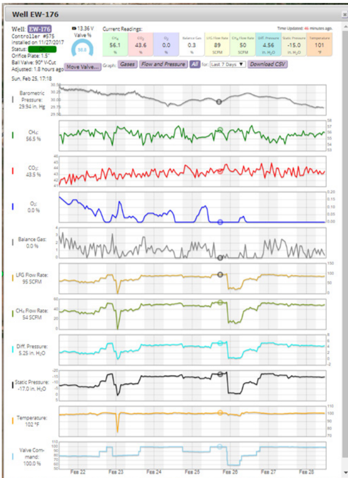
Photo 2: WellWatcher® user interface, with representative gas composition, flow, valve position; as well as 7 days of historical data on gas collector EW-176, at the Oklahoma City landfill.
